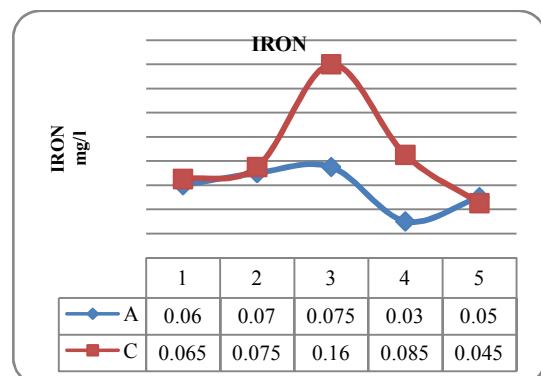
Fig 10 Iron Analysis
